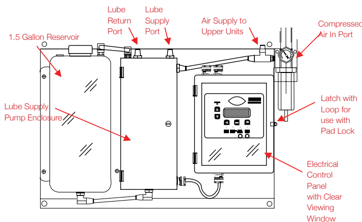
Lower Supply Pump & Controls
