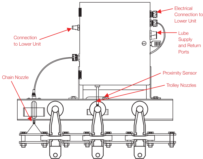
Upper Lubricating Head
